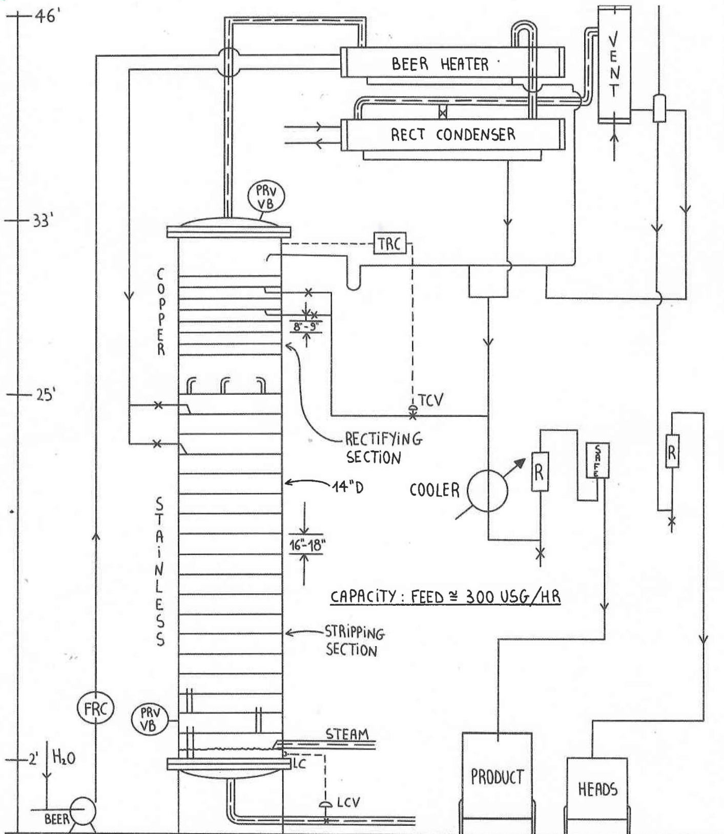
SCHMATIC FOR 14" D BEER COLUMN TO PRODUCE BOURBON STYLE, RUM, WHISKEY * FEED AT 7% ABV. # OF TRAYS IN RECT CAN BE REDUCED. 300 USG/HR → A2 USPG/HR
